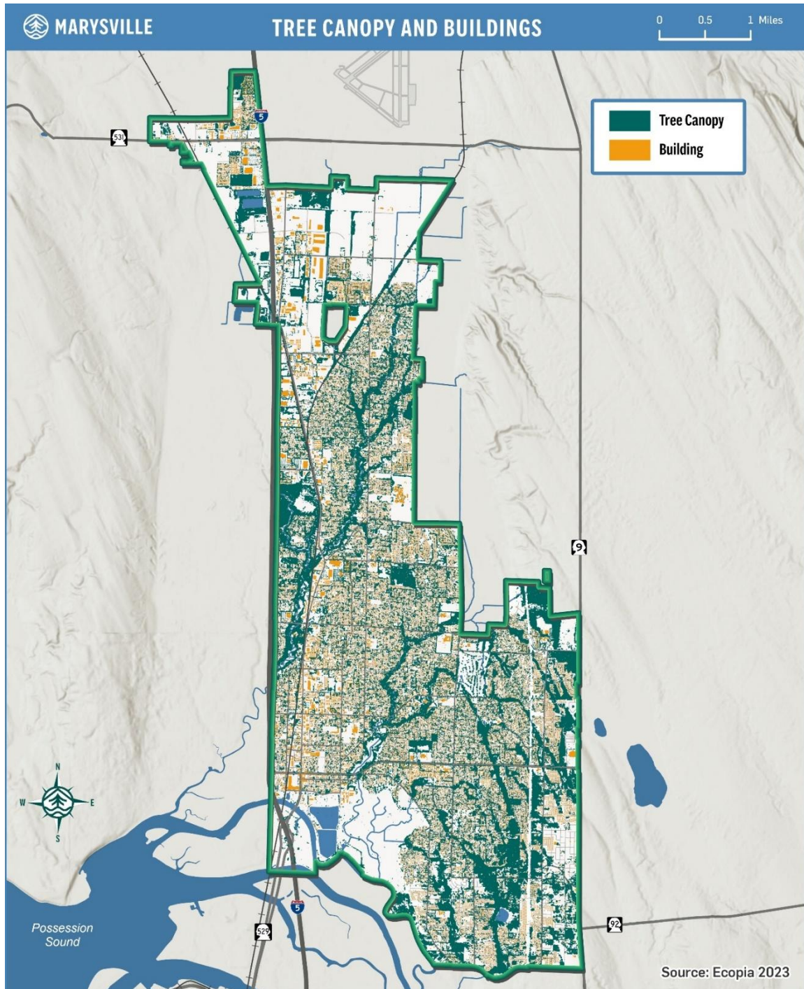
Figure 17. Tree Canopy Map
