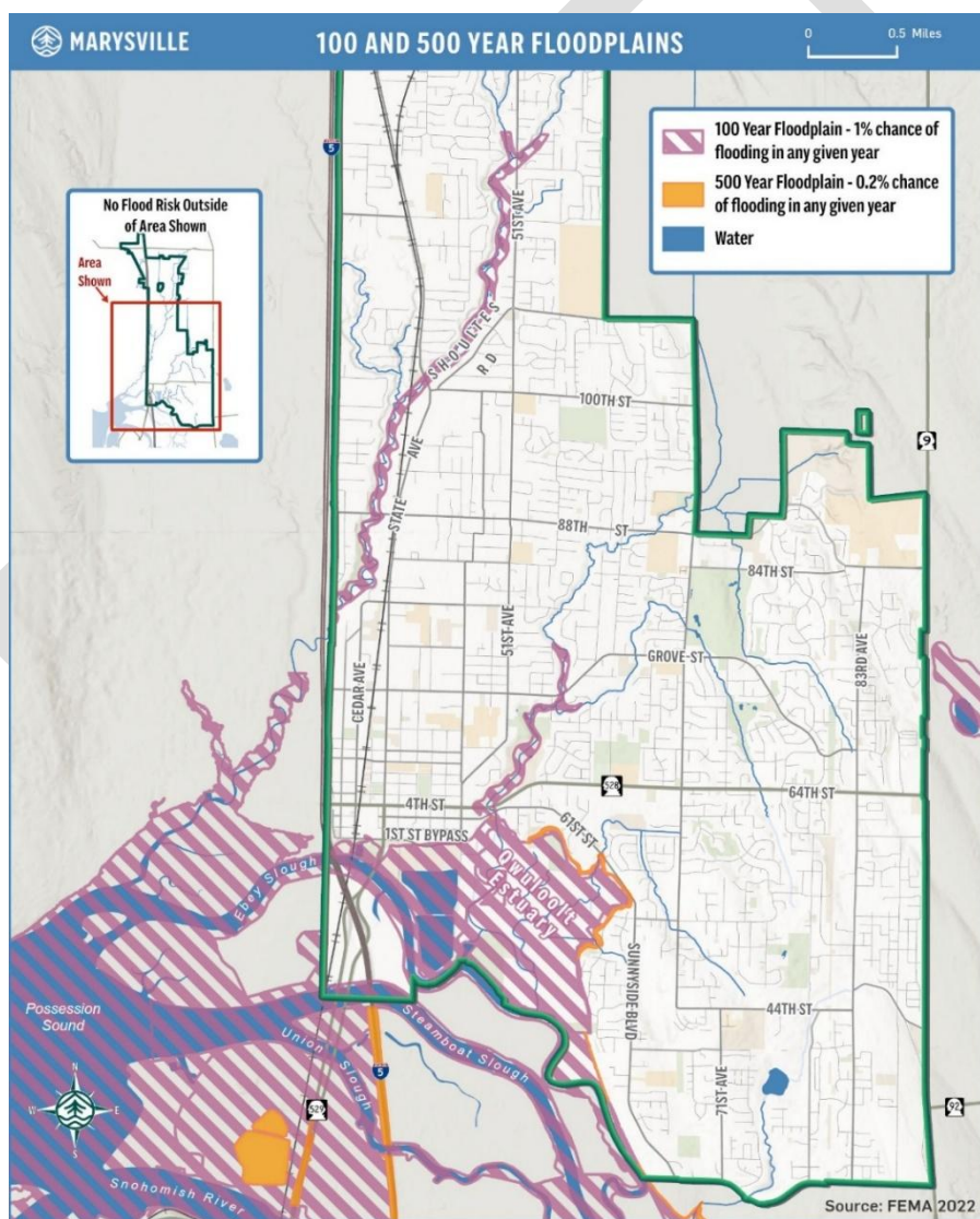
Figure 13. 100- and 500-Year Floodplains
