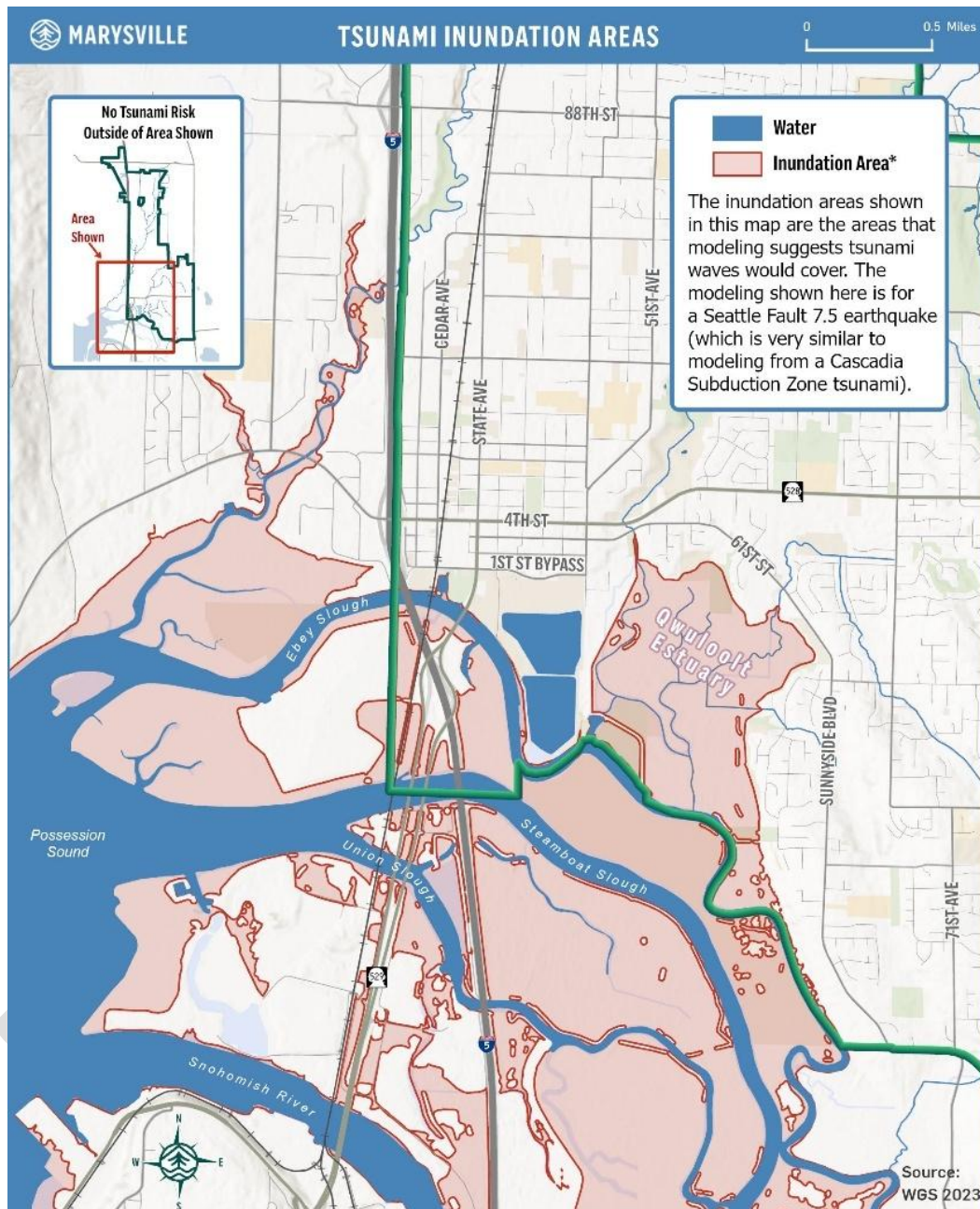
Figure 15. Tsunami Inundation Areas
