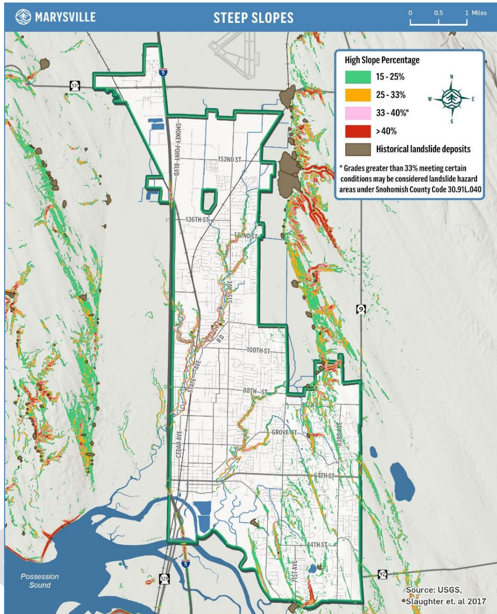
Figure 14. Steep Slopes
