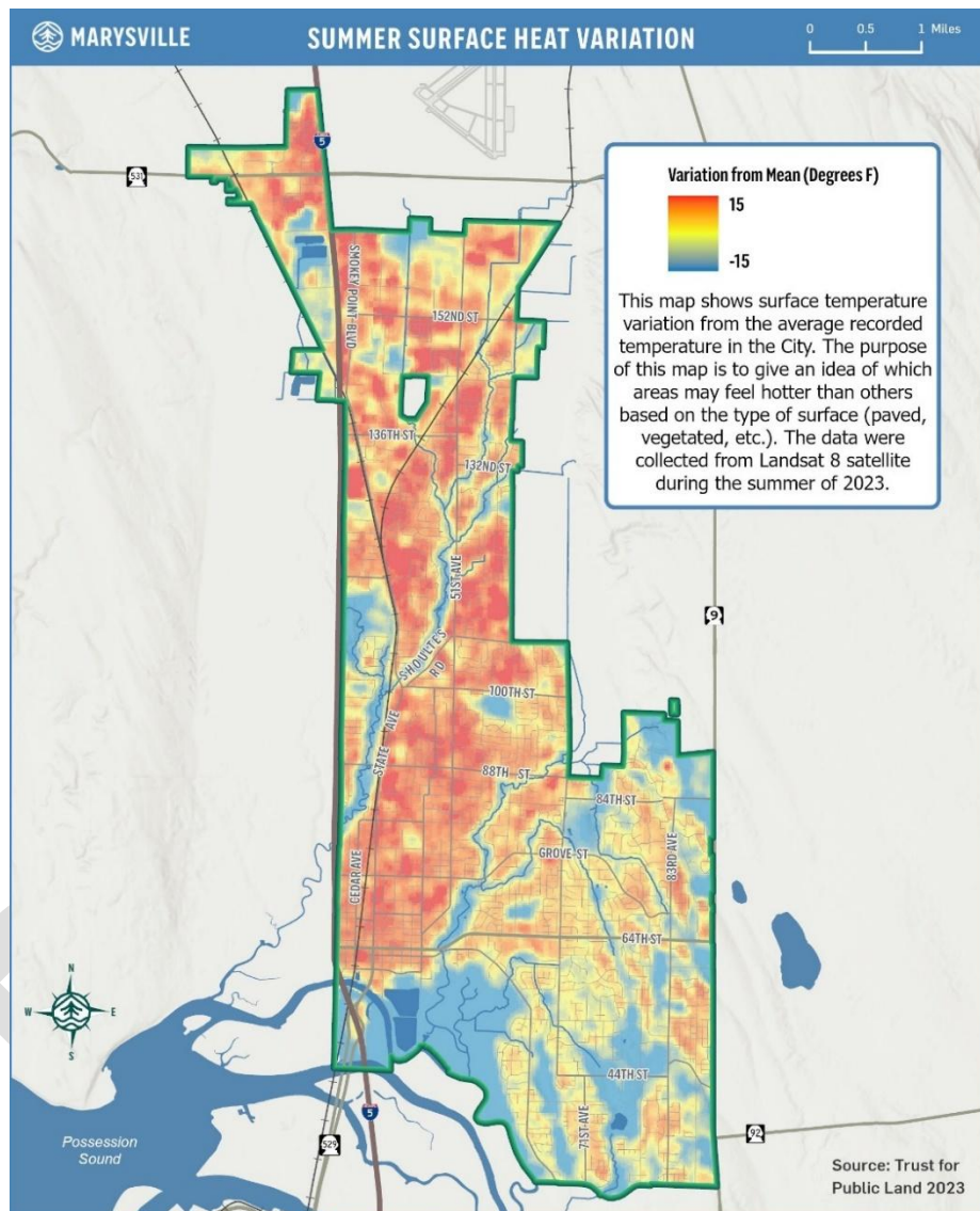
Figure 12. Summer Surface Heat Variation
