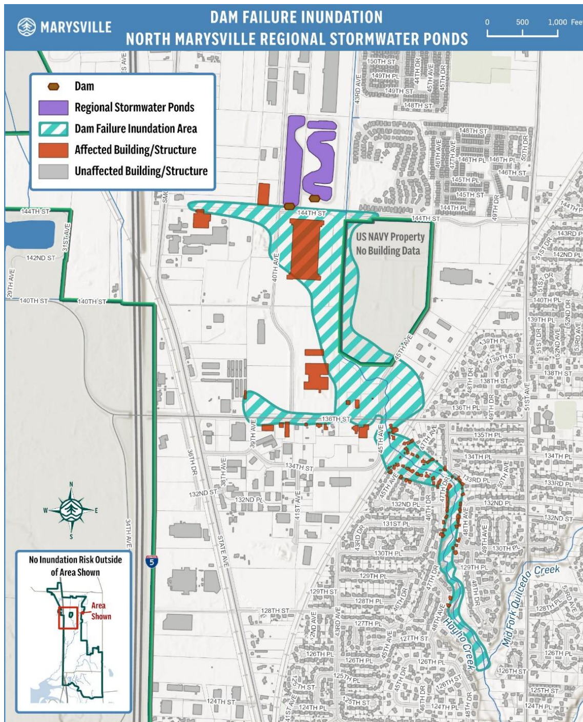
Figure 20. Dam Failure Inundation Map for North Marysville Regional Stormwater Ponds
