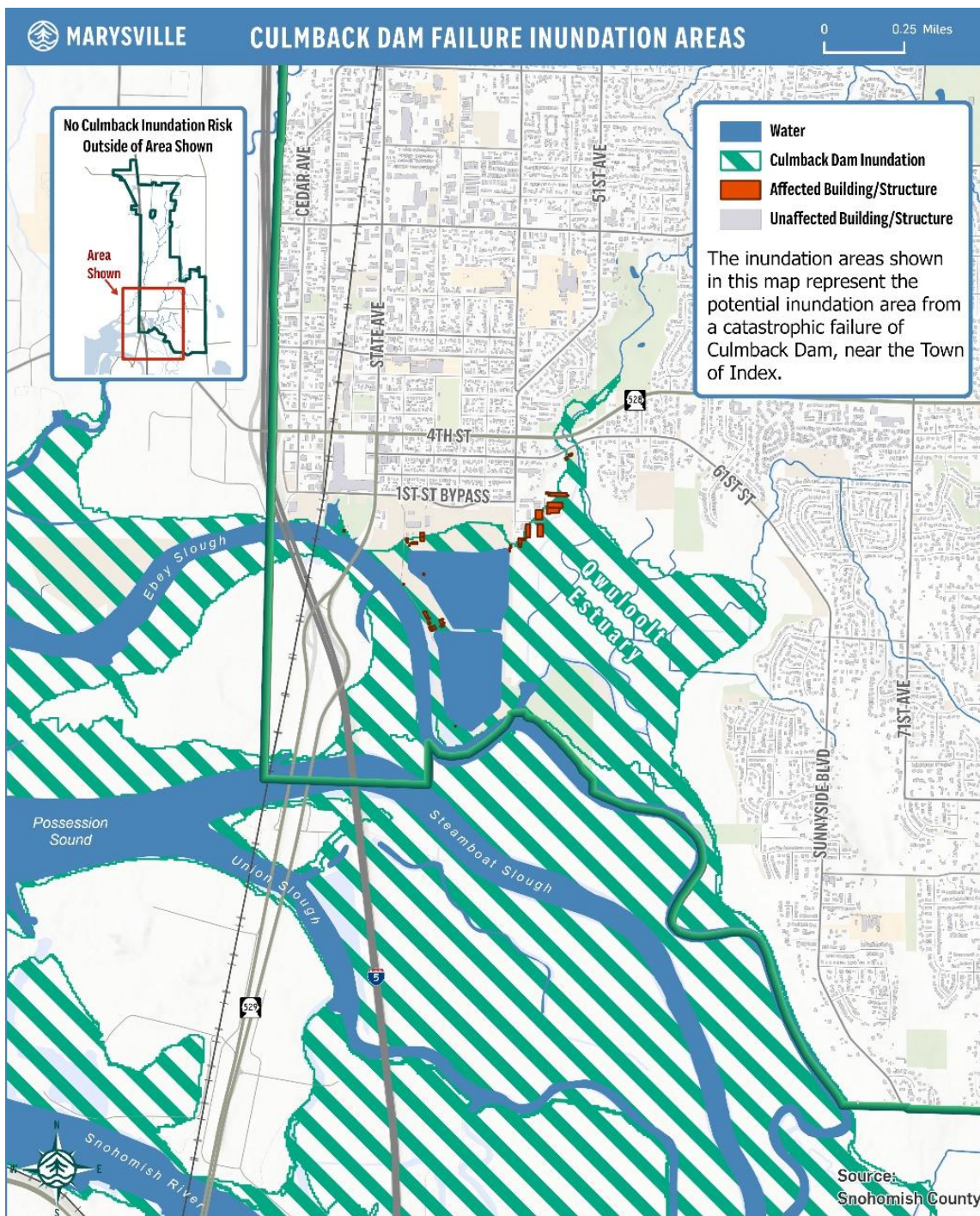
Figure 21. Dam Failure Inundation Map for Culmback Dam
